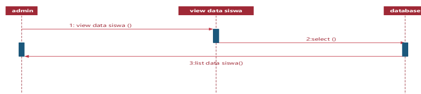
Gambar 1.8 Sequence Diagram Menu Siswa Admin
