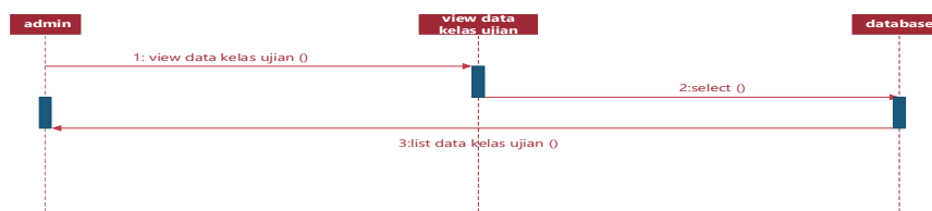
Gambar 2.1 Sequence Diagram Menu Kelas Ujian Admin
