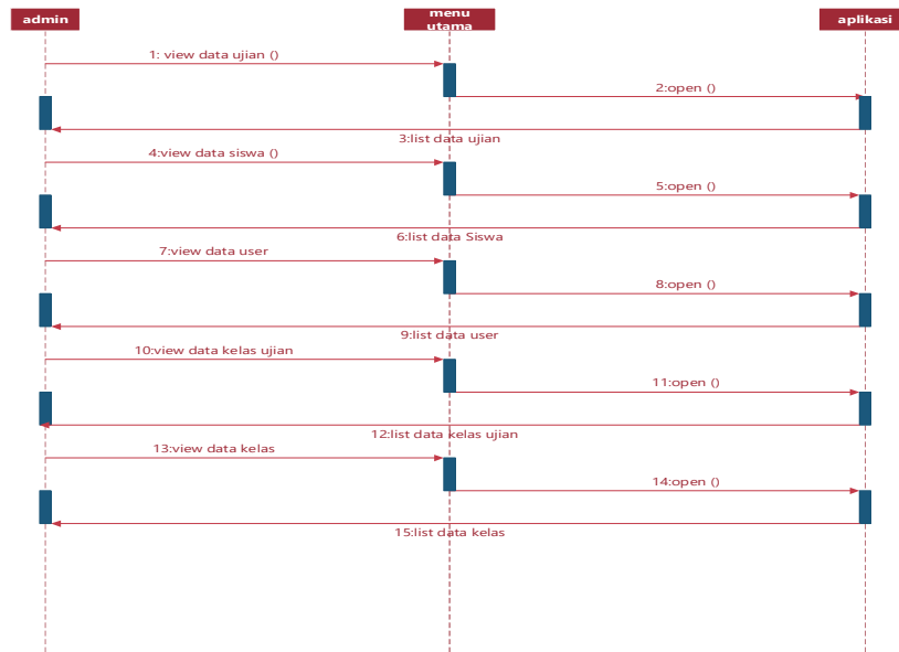
Gambar 1.6 Sequence Diagram Menu Utama Admin
