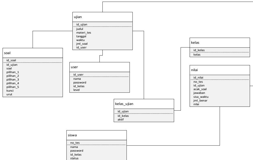
Gambar 1.8 Class Diagram Databases
