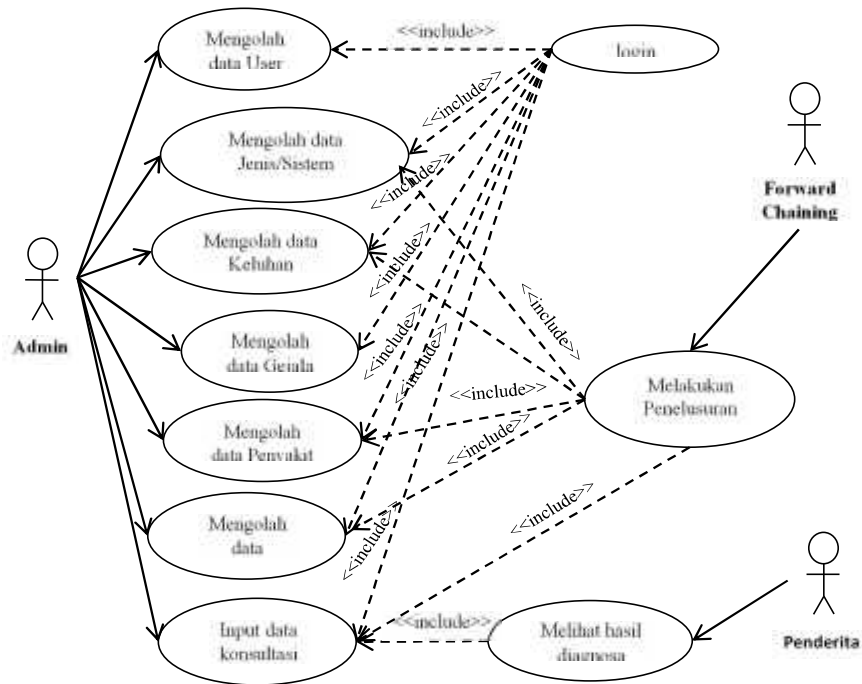
Gambar 2. Use Case Diagram Sistem Pakar ThibbunNabawi
